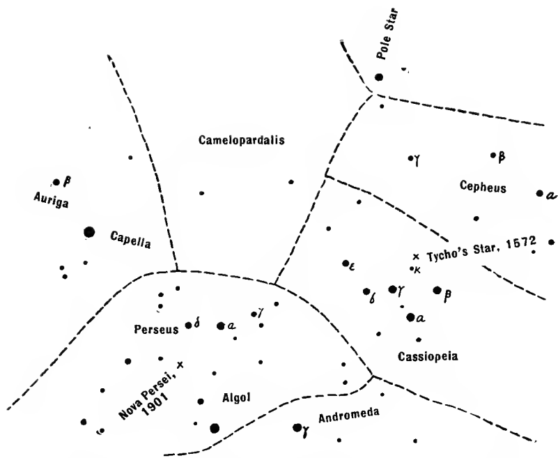
CHART SHOWING LOCATION OF TYCHO'S STAR, 1572, AND NOVA PERSEI OF 1901
